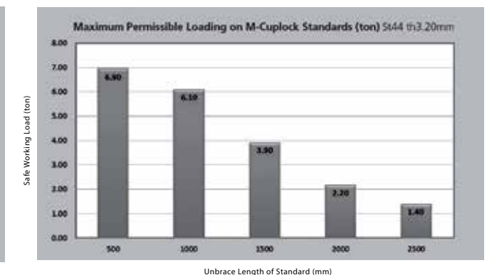
D- For tubes 48.3mm dia, Thk 3.2mm and steel 44
