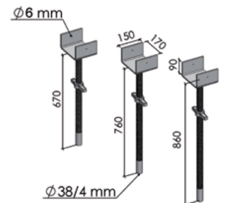
Adjustable U-head Jacks Hollow
