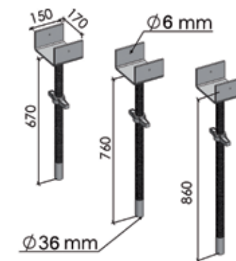
Adjustable U-head Jacks Solid
